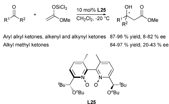
Scheme 22 Enantioselective aldol reaction between trichlorosilyl ketene acetal and ketones catalysed by a chiral bis N -oxide Lewis base catalyst developed by Denmark et al. (2002).
