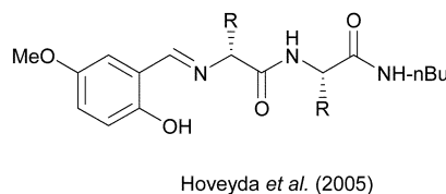
Fig. 3 Chiral ligands developed for enantioselective alkylation of ketones.
