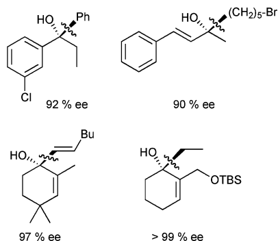
Scheme 5 Walsh's catalytic method for the asymmetric addition of functionalised organometallics to ketones.
